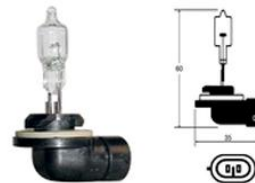
HELLA-881 FOCO 12V 27W BASE PGJ13 ESCUADRA
