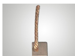
FA-111 Hitachi Starter WAI # 68-8100 DD, OSGR 12V
